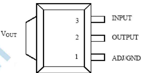
A Package (SOT-89)
